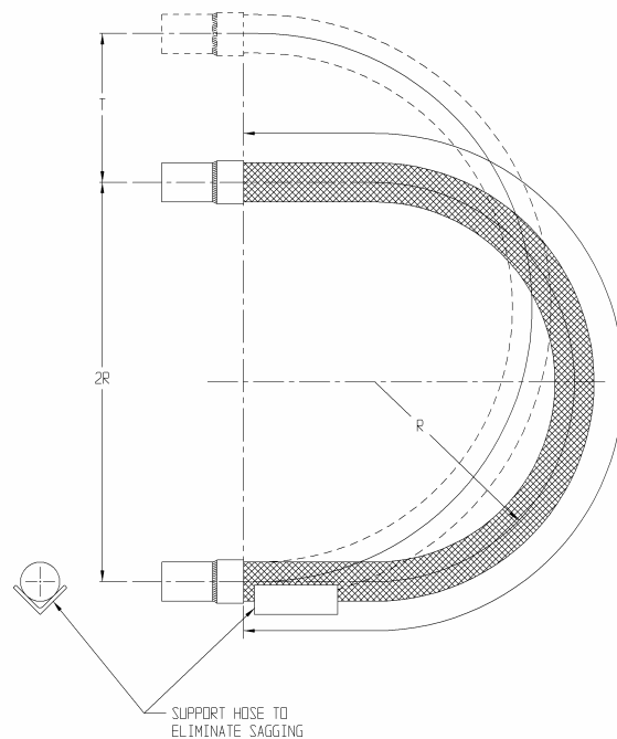
Figure 3.6.5.1 Variable Radius Traveling Loop - Vertical Travel
