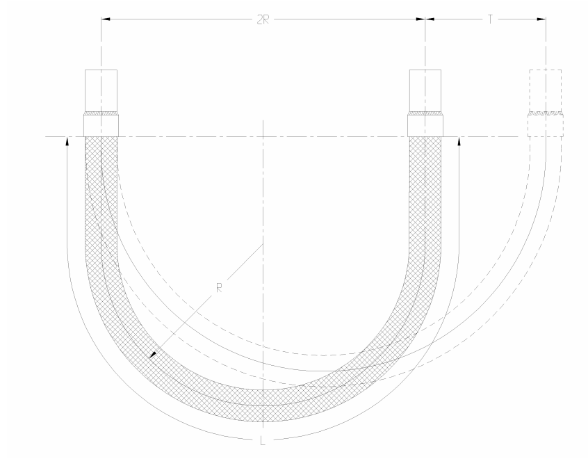
Figure 3.6.5.2 Variable Radius Traveling Loop - Horizontal Travel
